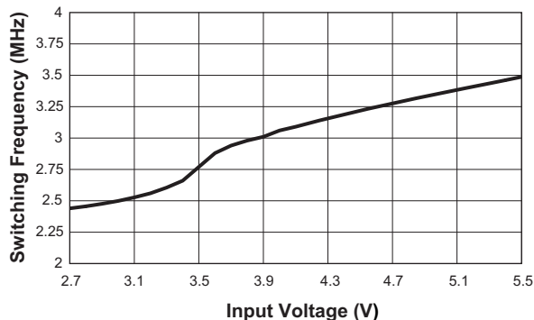
Switching Frequency vs. Input Voltage (V OUT = 1V; C IN = C OUT = 2.2µF; L = 1µH)
